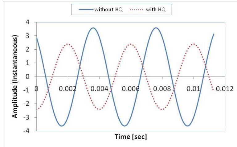
Figure 11. Time history of the acoustic signals, without and with a long HQ at frequency of 250 Hz.
